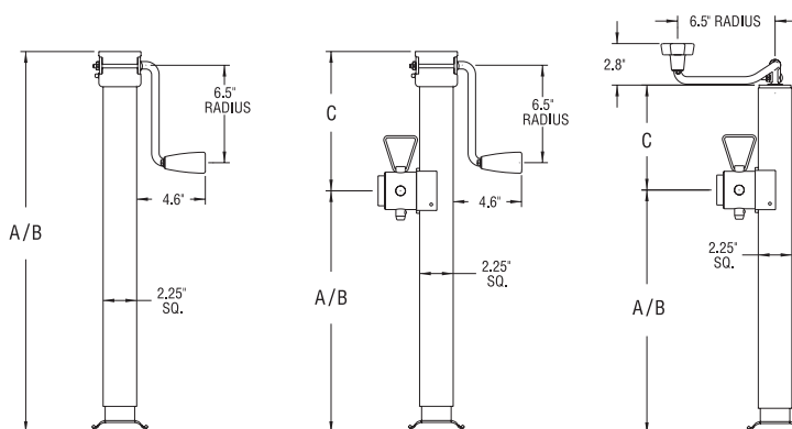
Travel and Clearance Diagram
