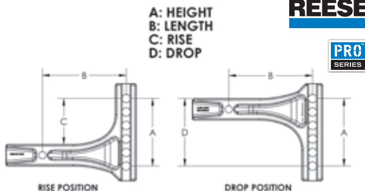
How to measure for the proper hitch bar (Illustrations show Adjustable Hitch Bar)
